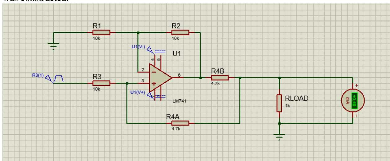
Figure 1. Circuit Simulation
