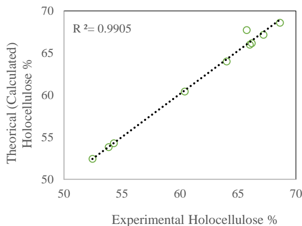
Figure 1. Relationship between experimental holocellulose content and calculated holocellulose value.
