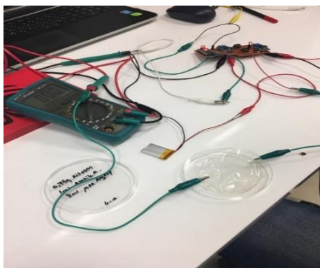
Figure 8. Groups current measurements
