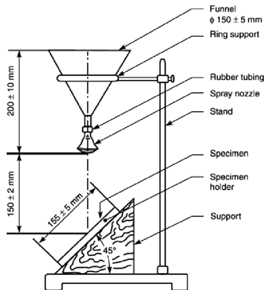
Figure 1. Schematic diagram of a typical spray test for testing water repellency of
